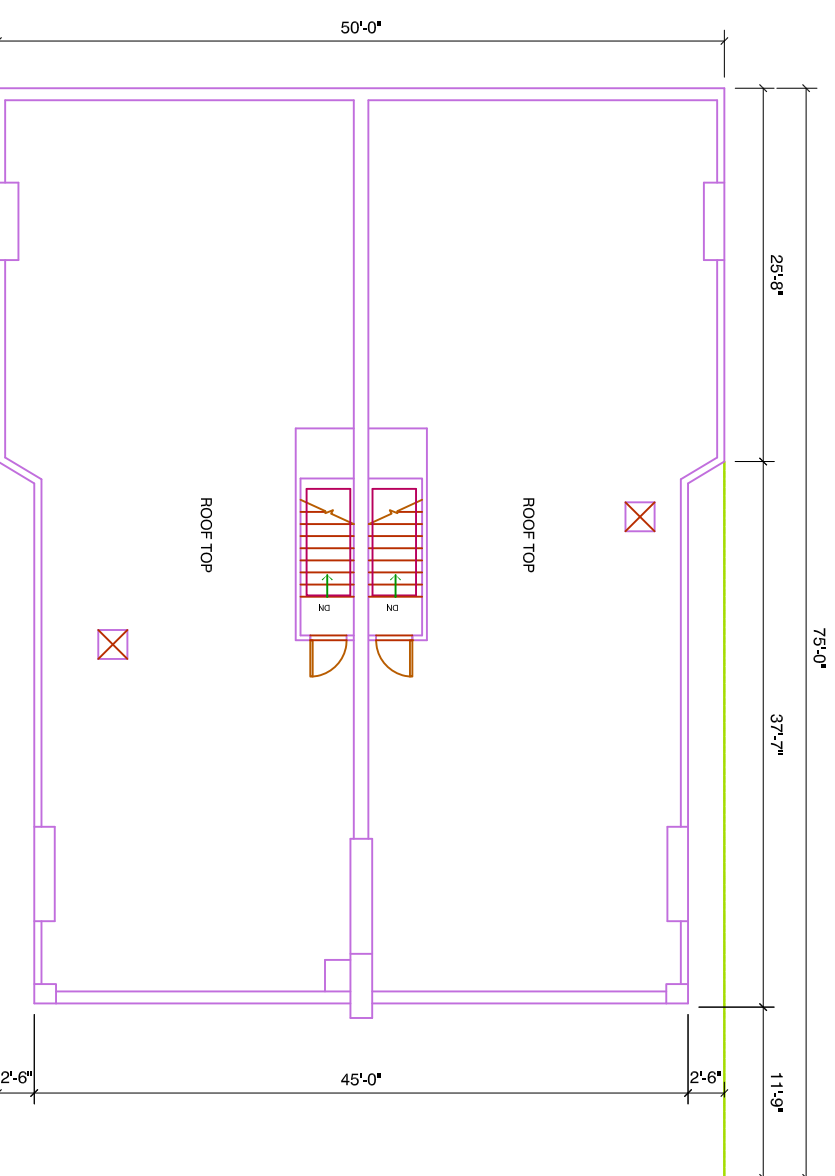
4 ROOF PLAN SCALE: 1/4"=1'-0"
