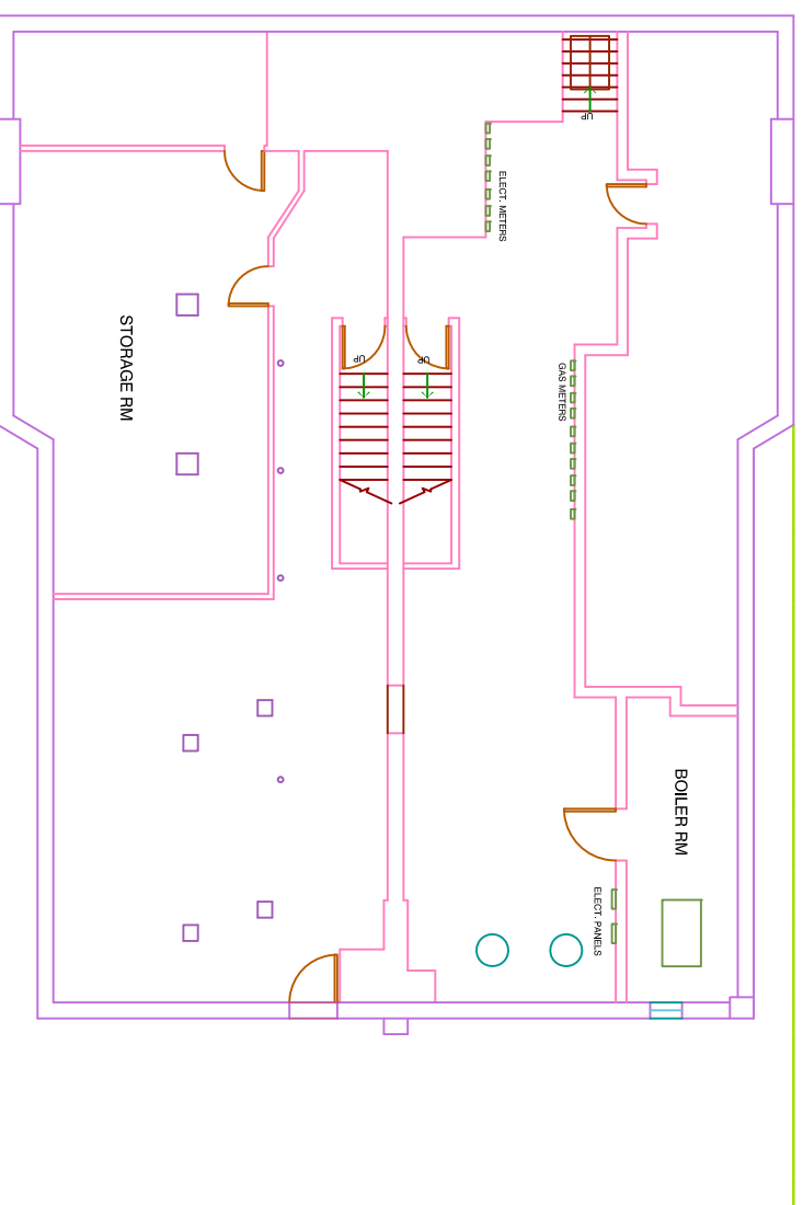
1 CELLAR PLAN SCALE: 1/4"=1'-0"
