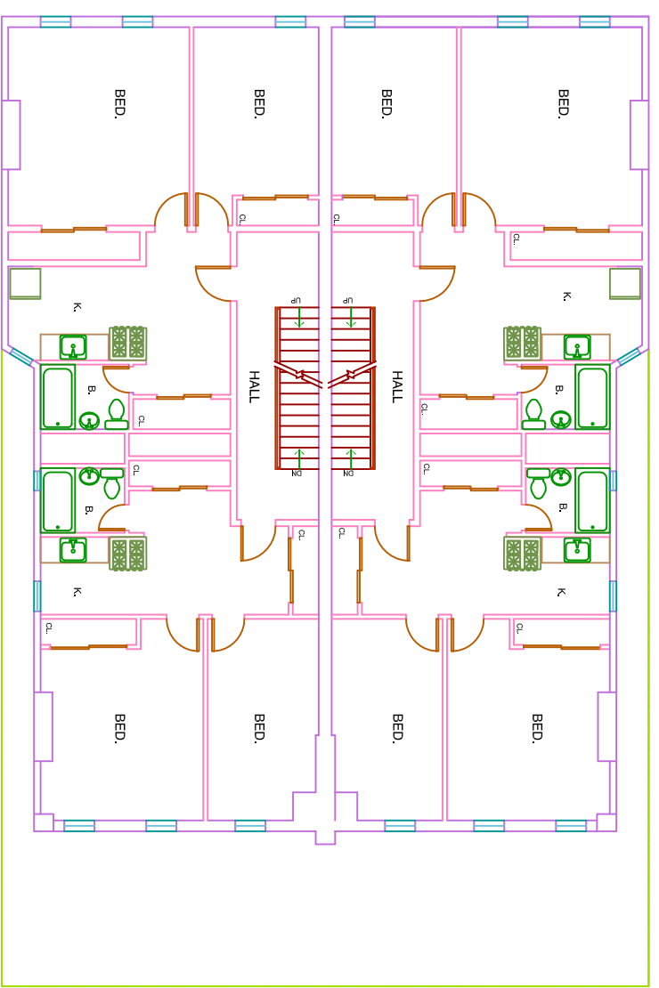
3 TYPICAL FLOOR 2ND-4TH PLAN SCALE: 1/4"=1'-0"
