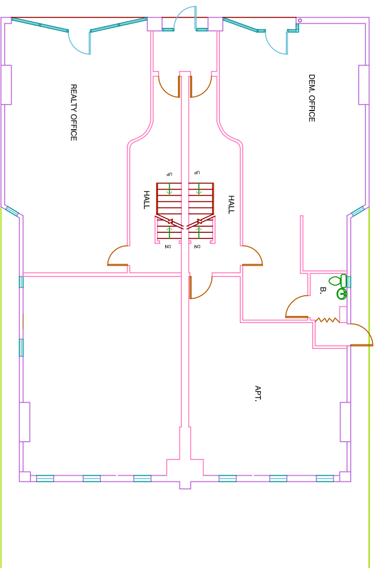
2 GROUND FLOOR PLAN SCALE: 1/4"=1'-0"
